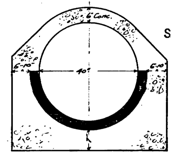
Section of 40" Cir. Conc. Scale 1/2" = 1'
