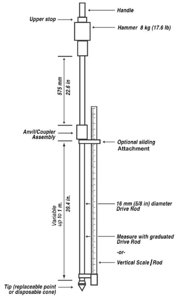
Figure 1 - Schematic of DCP Device
