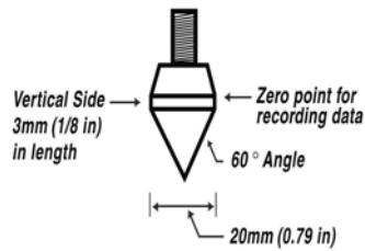
Figure 2 - Replaceable Point Tip
